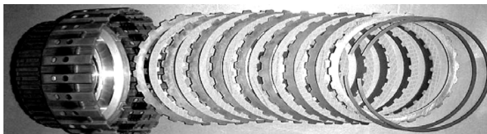
Direct Drum/ Clutch Pack
