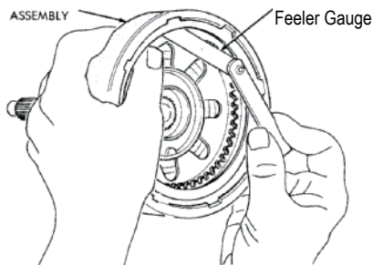
Rear Clutch Assembly
